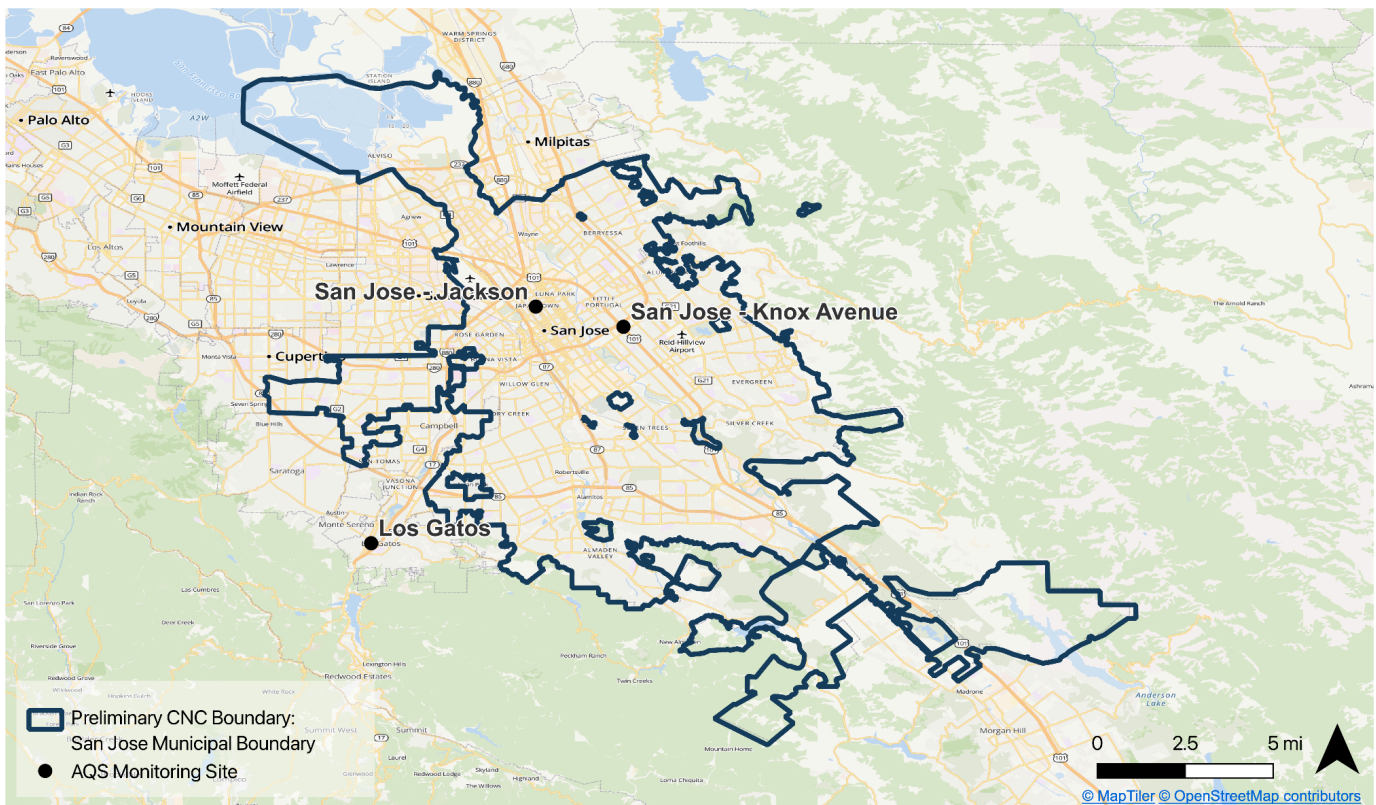
Figure 2.2: San Jose municipal boundary and local Air Quality System (AQS) monitoring sites.
