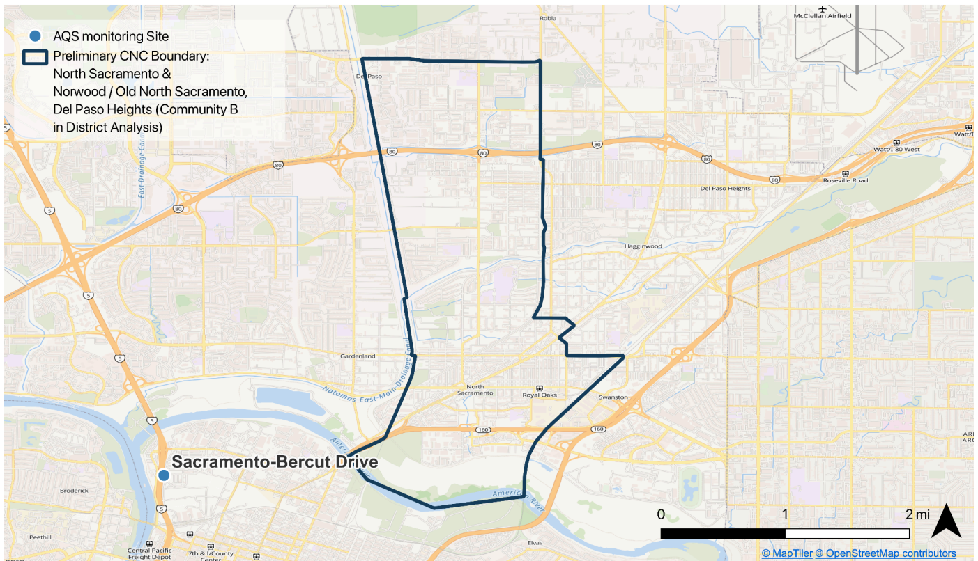
Figure 2.2: Preliminary CNC boundary for North Sacramento and Norwood / Old North Sacramento, Del Paso Heights (Community B in District Analysis), and the nearby Sacramento-Bercut Drive local Air Quality System (AQS) monitoring site.
