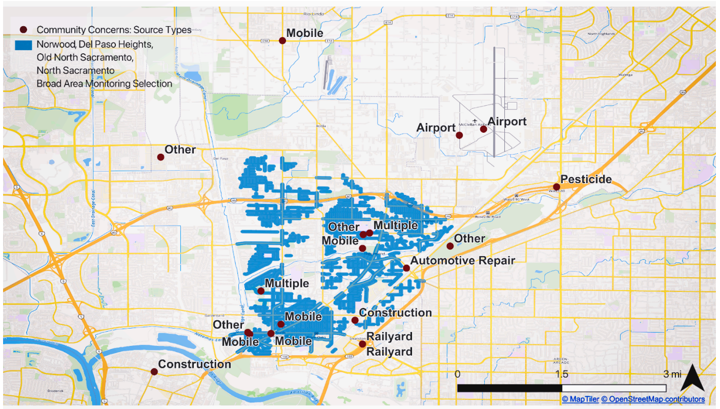
Figure 8.1: Map of the Norwood, Del Paso Heights, Old North Sacramento, North Sacramento final community Broad Area Monitoring selection and local air quality community concerns. Concerns noted by this CNC’s community members include the airports to the northeast of the CNC, a railyard, mobile sources, automotive repair, and a number generally impacted neighborhoods.
