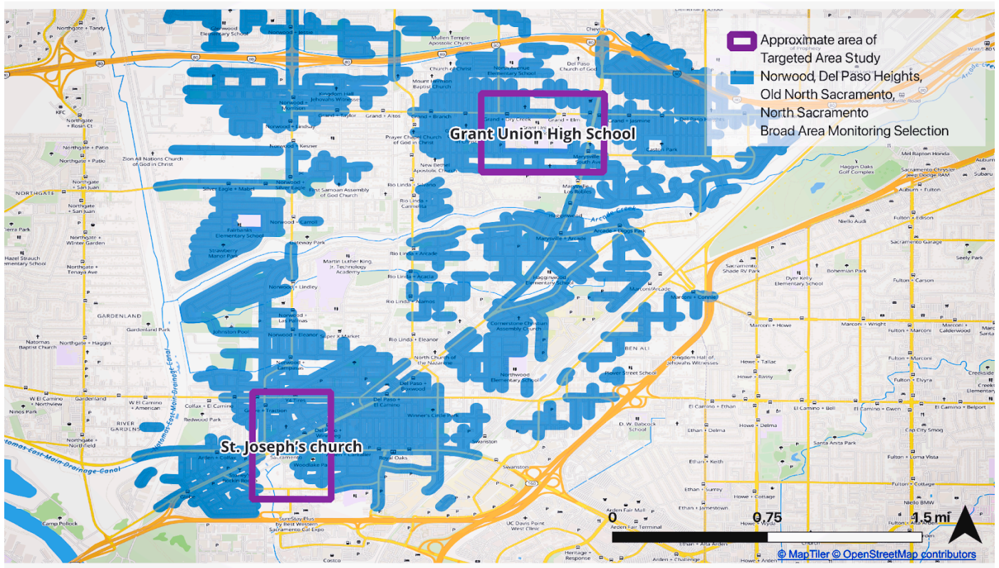
Figure 8.4 Map showing general area for the targeted area study (area around Grant Union High School in Hagginwood to the north, and near St. Joseph's Church to the south). Actual drive plan and extent of monitoring is to be determined and may change in response to conditions experienced during the monitoring. See text for description of the monitoring approach.
