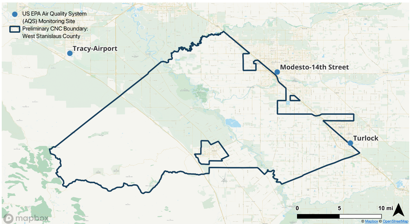
Figure 2.2: West Stanislaus County preliminary CNC boundary and local Air Quality System (AQS) monitoring sites.
