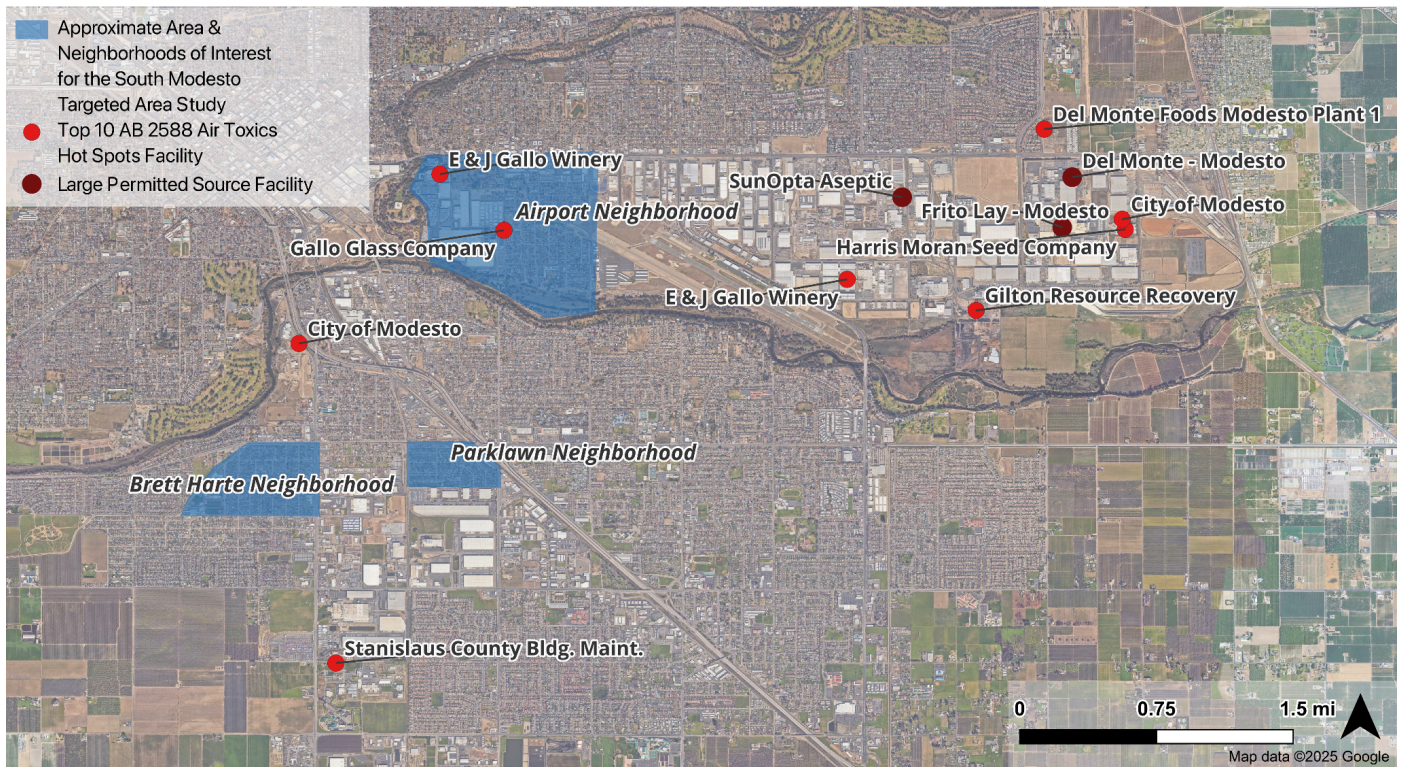
Figure 8.5: Map showing general area for the targeted area study. Actual drive plan and extent of monitoring is to be determined.
