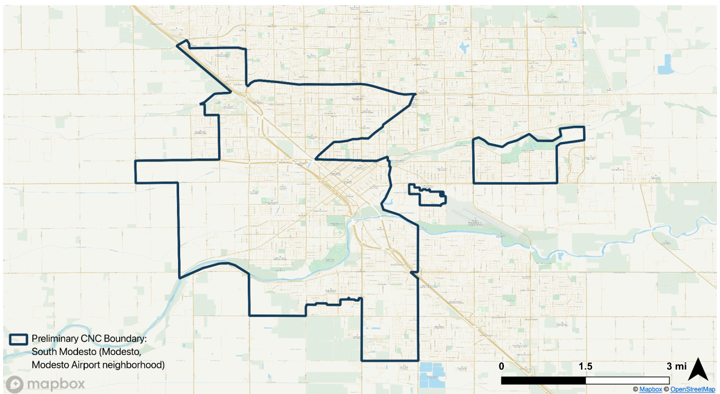
Figure 2.1: Preliminary CNC Boundary: South Modesto. Preliminary boundary based on Modesto census tracts with a CES4.0 percent score \geq 75 and the municipal boundary of the Airport Census Designated Place (CDP).
