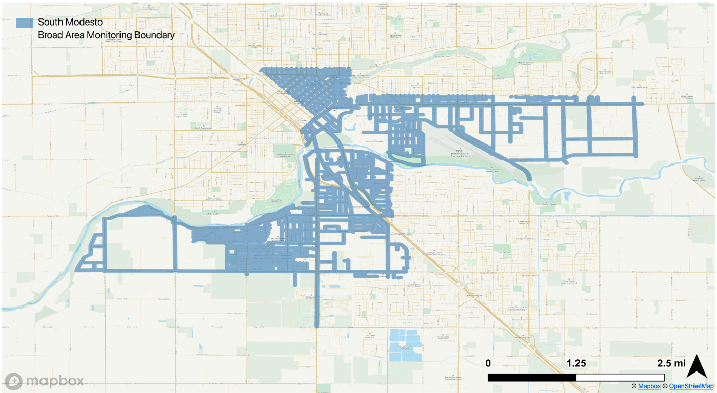
Figure 8.1: Map of the broad area monitoring boundary selected by South Modesto community members.
