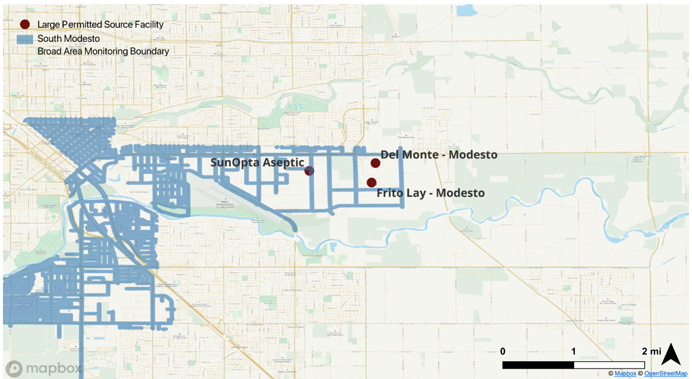
Figure 8.4: Map of large permitted facilities within and near the South Modesto broad area monitoring boundary. Pollutants reported by these facilities include methane, PM_{2.5} , PM_{10} , NO_x , and SO_x emitted as a result of these facilities' large-scale combustion processes.
