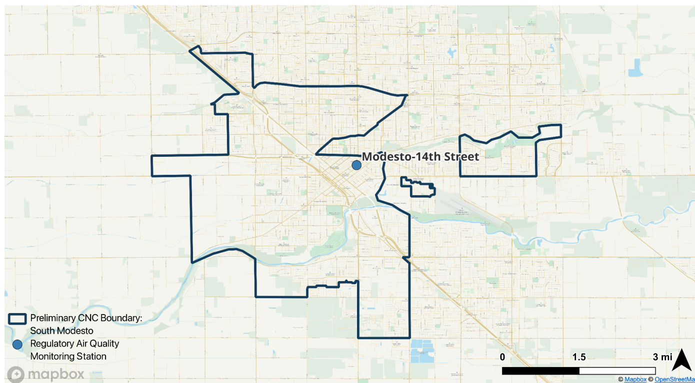
Figure 2.2: Map of the preliminary South Modesto CNC boundary and a local regulatory air quality monitoring site.
