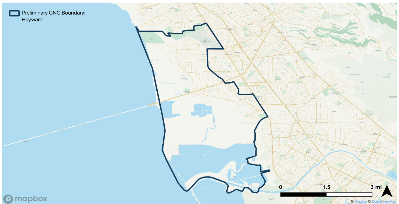
Figure 2.1: Preliminary Hayward CNC Boundary
