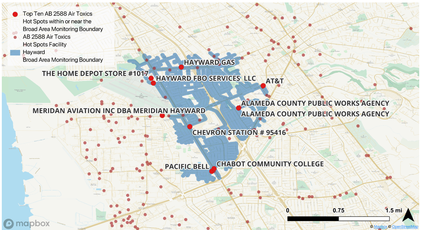
Figure 8.3: Map of AB 2588 Air Toxics Hot Spots within and near the Hayward broad area monitoring boundary. The top 10 hot spots, based on total toxicity-weighted emissions (TWE), are emphasized. These sources include public agencies, educational institutions, petroleum wholesalers, telecommunications companies, and gasoline service stations.
