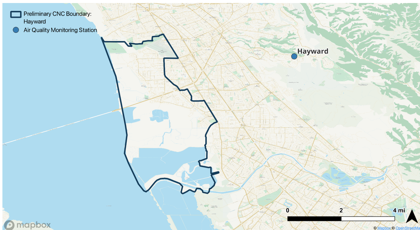
Figure 2.2: Map of the preliminary Hayward CNC boundary and local US EPA Air Quality System (AQS) monitoring sites.
