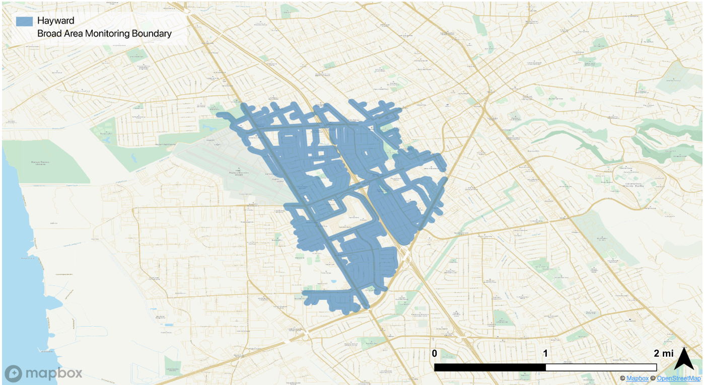
Figure 8.1: Map of the area for mobile monitoring in Hayward.
