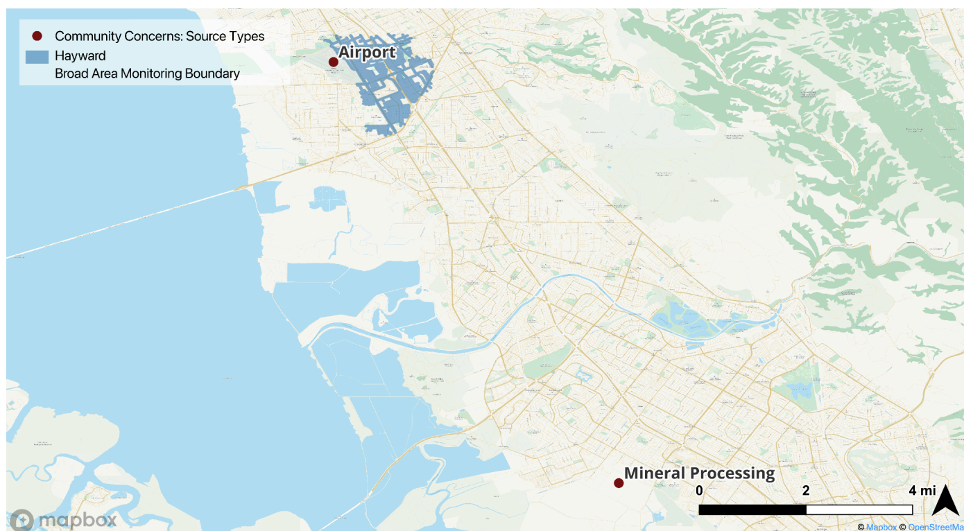
Figure 8.2: Map of the Hayward broad area monitoring boundary and local air quality community concerns. Concerns noted by Hayward community members include Hayward Airport, a mineral processing plant, and (though not shown in this figure) major traffic corridors such as Highway 880 and State Route 238.
