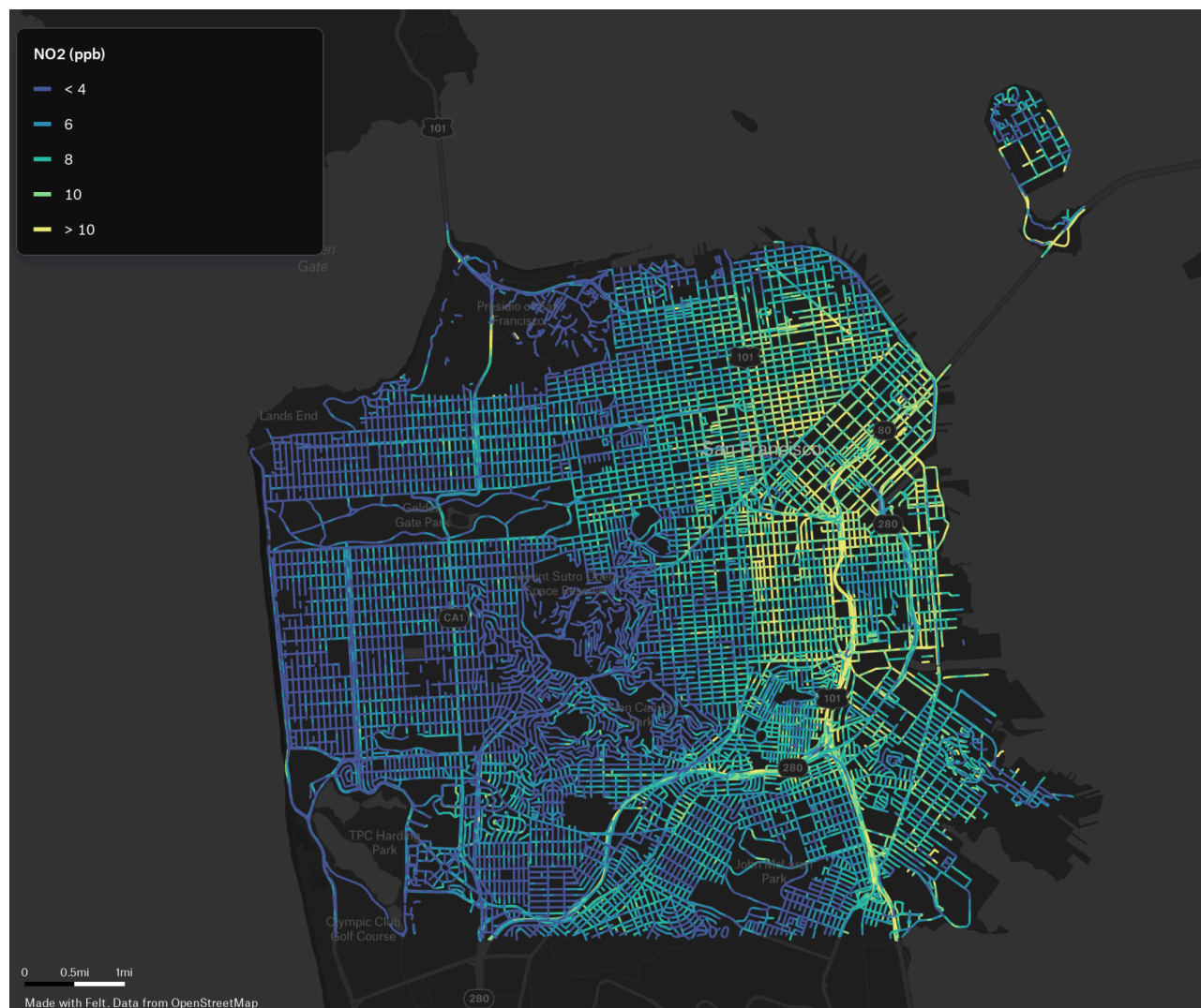
Figure 4.1: Example of plotted ambient concentration estimates for \text{NO}_2 in the San Francisco Bay Area, CA, showing typical concentrations observed over a 1-year monitoring period. This example shows how high \text{NO}_2 concentrations (as illustrated by the brighter green colors) are disproportionately impacting the eastern parts of the city. This plot uses data generated by the broad area monitoring method.
